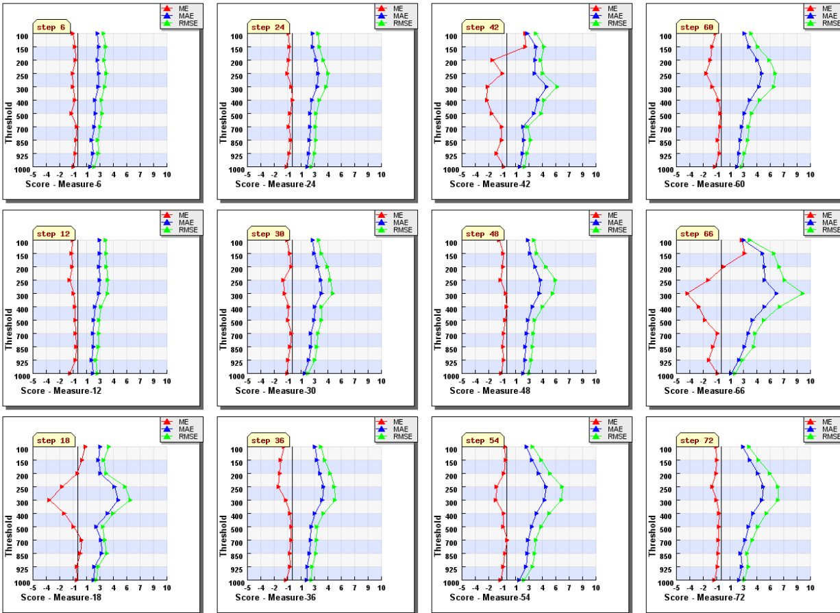
COSMOME Seasonal Run 00 Wind speed - Italy - 00 Run Stratification : All Italian TEMP Station - Period: JJA 2010
