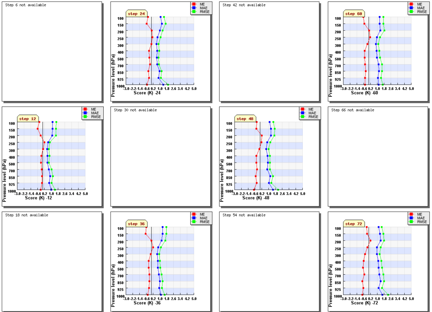
COSMO-ME Seasonal TEMPERATURE - Italy - 00 Run Stratification : All Italian TEMP Station - Period: DJF 2015-2016
